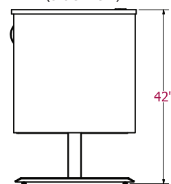
Sit-Stand Lectern in standing position (Side View)
