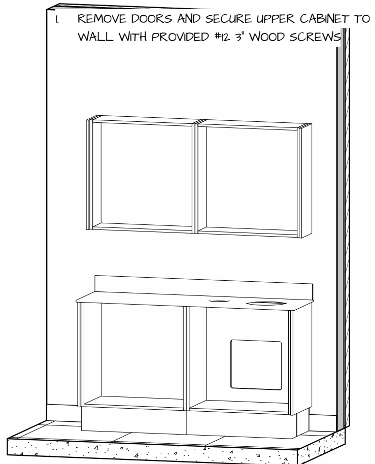
2.3 Install Upper Cabinets
