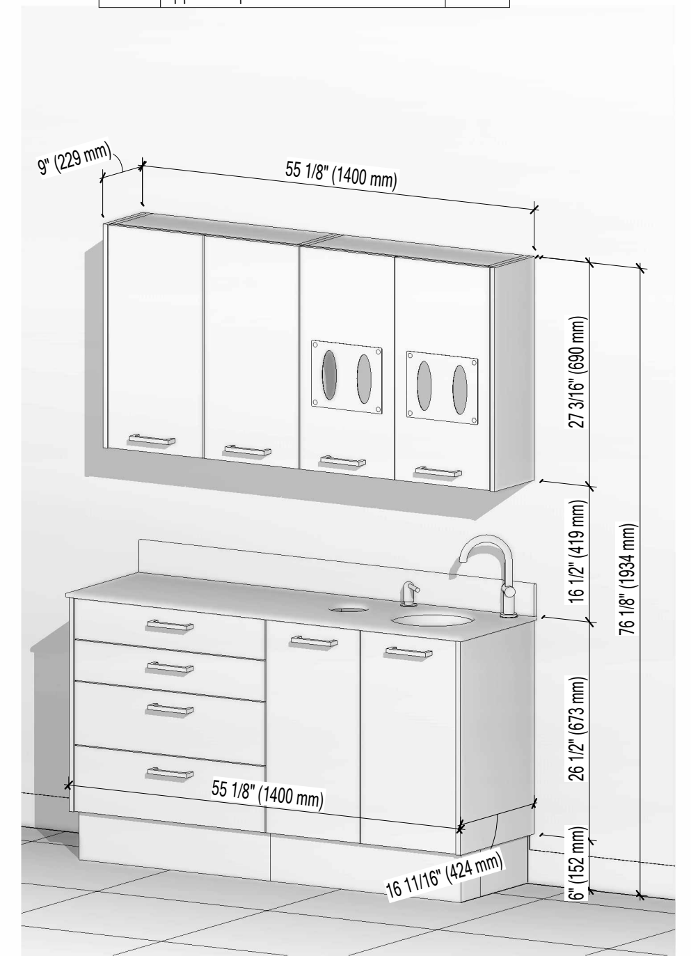
3 Final Installation View
