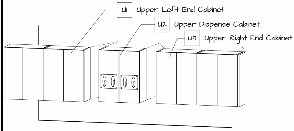
2.1 Install Upper Cabinets #14 1/2" Cabinet Screws
